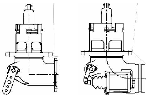
Air or Cable Operated Groove or Flange Outlet Buna Urethane or Viton Seals
