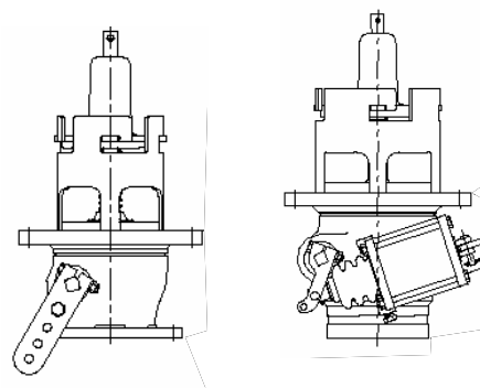
Air or Cable Operated Groove or Flange Outlet Buna Urethane or Viton Seals
