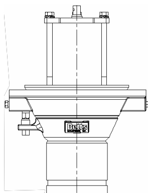
6" Straight
