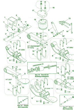
Hendrickson Trailer HK/HS 190/230 HT 190/230/250/300 Appendix H-3
