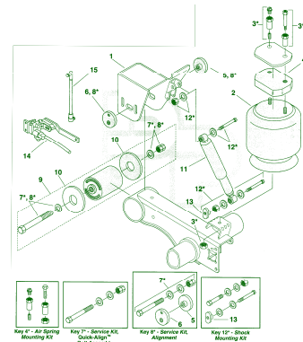
Hendrickson Trailer Intraxx/Vantraxx AA230/250T, HKA180/200/250 Trailer Air Suspension Appendix H-9
